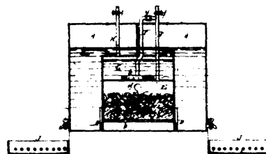
2690 Wainwright's Gas Apparatus.
