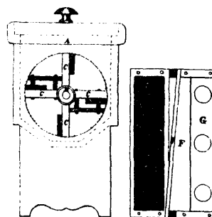
4480 Blamey &amp; Kulow's Churn.
