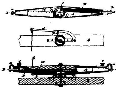
4488 Edwards &amp; Rowe's Improvements on Whiffle Trees.
