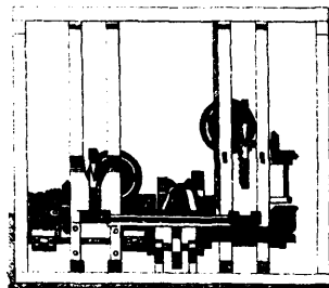
4487 Mayrand's Floating Mill and Machine for Splitting Cord Wood.
