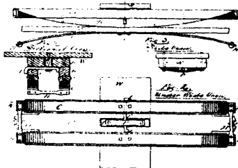
4478 Wright &amp; Krehbiel's Carriage Spring.
