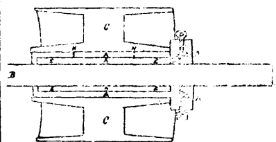
2017 Telfer's Oilier for the Shafts of Louse Pulleys and other Bearings.
