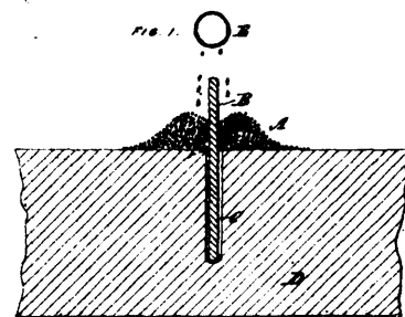
2020 Tilghman's Method of Cutting Hard Substances.
