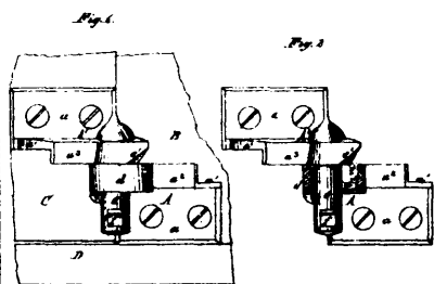
2021 Garretson's Blind Hinge.
