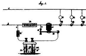
13906 Edison's Improvements in Meters for Measuring Electric Currents.
