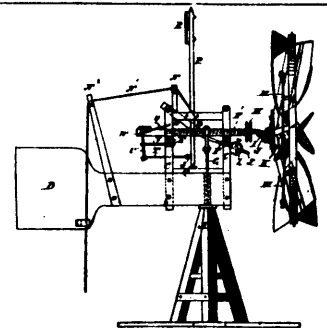
13913 Lee's Improvements in Windmills.
