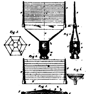
13904 Jackson's Improvements on Incandescent Burners.
