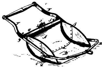
13903 Byrnett's Improvements on Earth Scrapers.
