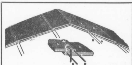
A shows method of laying Red Star Brand Wire-Edged Ready Roofing, with 2-inch laps secured by nailing two inches apart. BE shows wires running through the edges of the roofing, giving it great strength at the joints or laps—a very desirable feature, especially in localities where high winds prevail.
