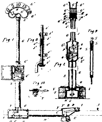
40450 Fountaine's Railway Time Signal.
