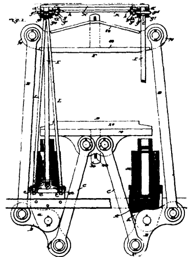
40452 Deane's Compound Press.
