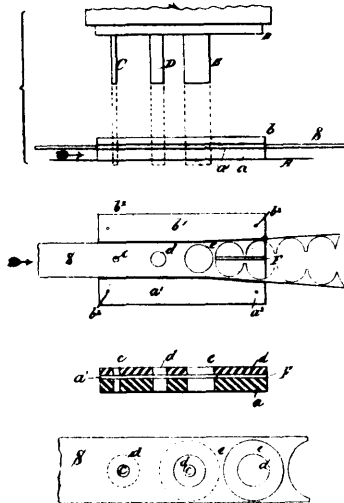
17714 Bronner's Metal Washer Making Machine.
