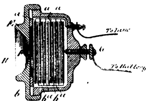
13363 Anders's Improvements in Telephones.
