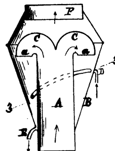
13359 McKenzie's Improvements on Spark Arresters.
