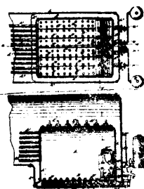
13368 Holland's Improvements on Hydro-carbon Burners.
