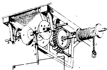
13371 Foster's Improvements in Hoisting Machines.
