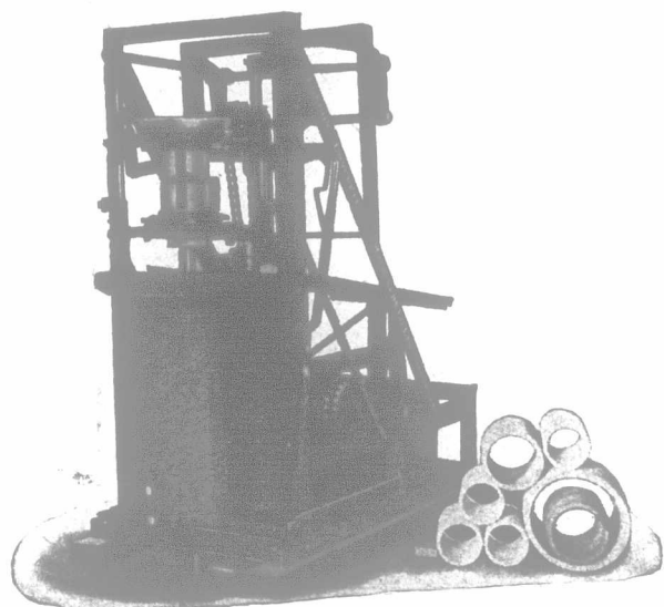
LONDON CEMENT DRAIN TILE MACHINE
