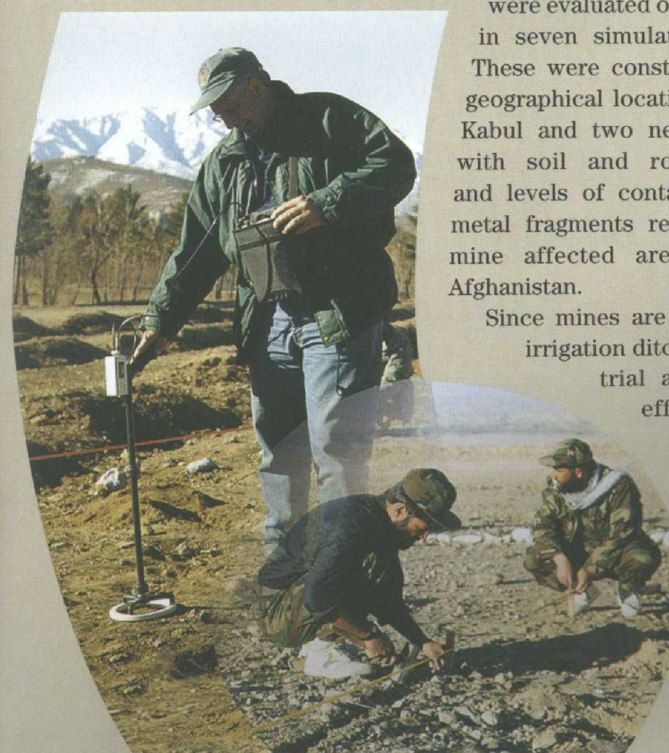
Testing detectors in a simulated, wet ground minefield in Afghanistan.
