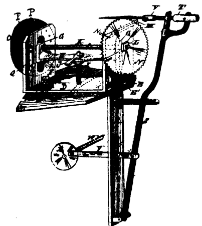
Chambers' Saw Filing Machine.
