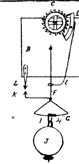
14026 Lash's Improvements in Clocks.
