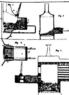
14033 Engert's Improvements on Fire Grates.
