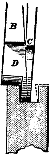
FIG. 2—CUTTER NEARLY USED UP.
