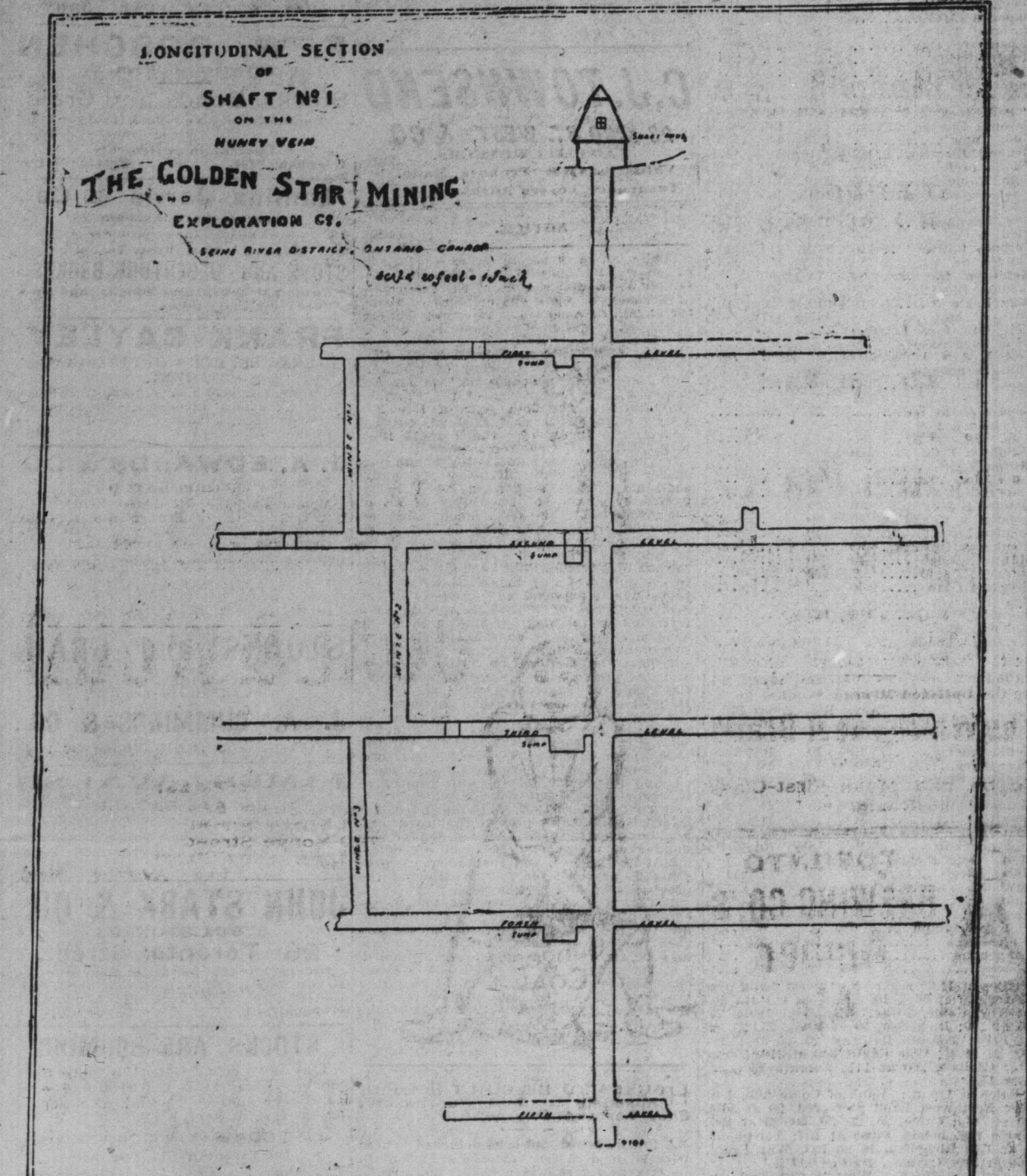
Working plans of Golden Star Mine, showing main shaft 400 feet deep, drifts at five levels aggregating 815 feet in length and 250 feet of winzes—in all nearly 1500 feet of underground workings.
