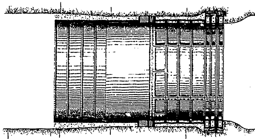
POSITION OF MOSS-BOX AFTER COMPRESSION, the Water Bottom being removed, and the Foundation Trenching and the Wedging-Blocks in Place.
