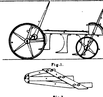
3855 Currie's Improvements on Gang Ploughs.
