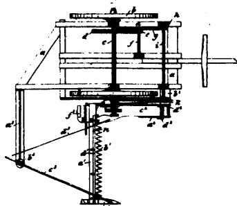
3851 Lockhead's Mowing and Reaping Machine.
