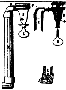
3854 Wellington's Hydro-carbon Burner.
