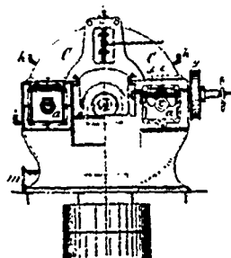
13708 Kaiser's Improvements on Wood Grinders.
