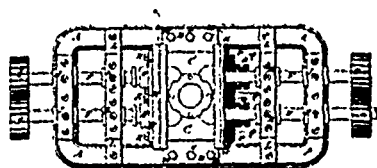
13695 Clark's Improvements in Rotary Pumps.
