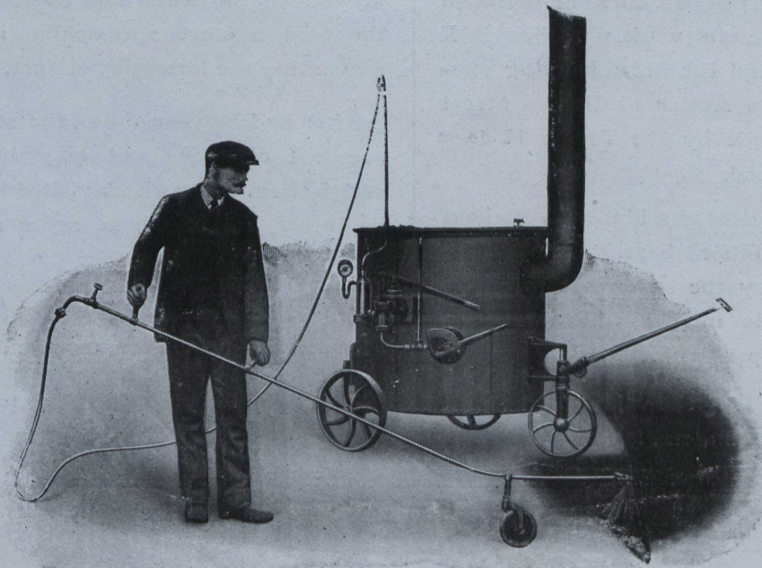
Vertical Tar Spraying Machine
