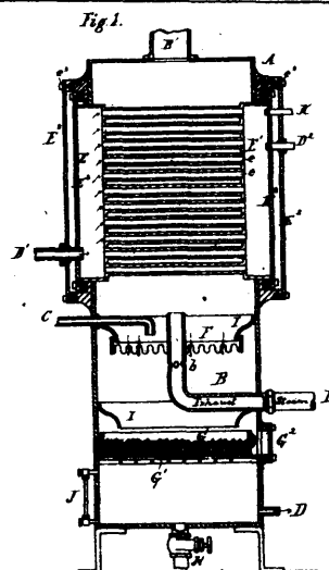
32583 Whitney's Culinary Utensil.
