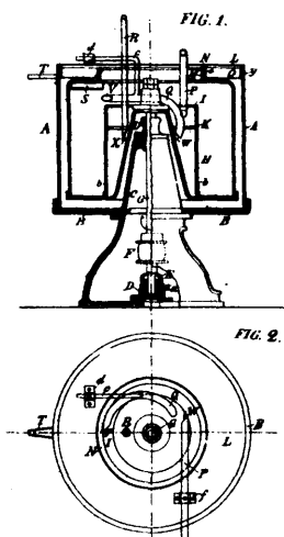
32585 Norliow's Apparatus for Manufacturing Butter.
