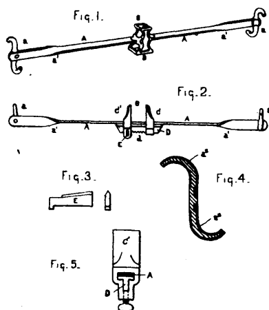
32581 Wegner's Carriage Wrench.
