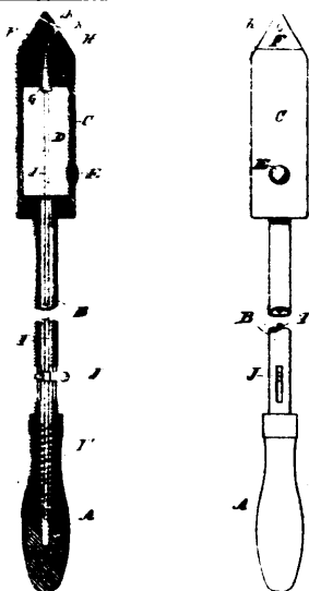
21557 Gillis &amp; McDonald's Soldering Tool.
