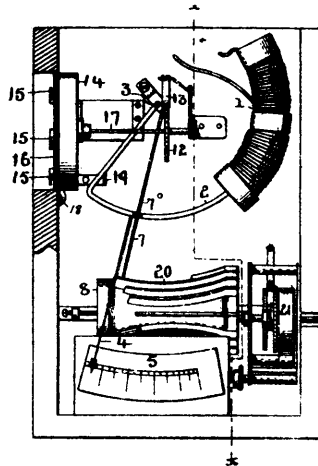
40750 Pilkington and White's Electrical Meter.
