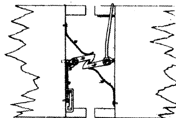
3431 Green's Improvements in Automatic Couplings for Railway and other Carriages.
