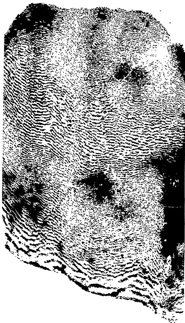
Fig. 2. Nature-printed specimen of Eozoon.
