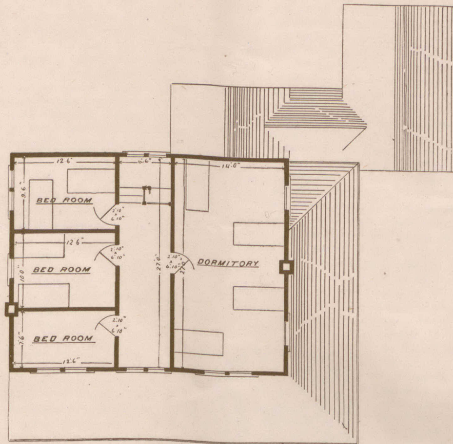
CHAMBER PLAN
