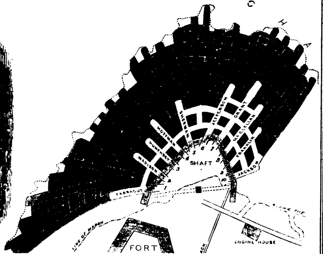
Fig. 3.—GROUND PLAN OF THE WORK AT HELL GATE.
