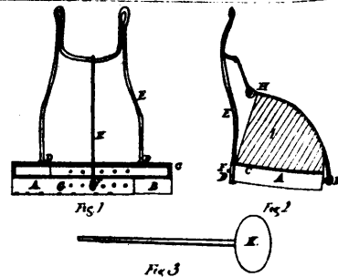
8505 Gibson's Potato Bug Gatherer.
