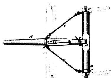
8508 Lawson's Improvement on Sled Poles.
