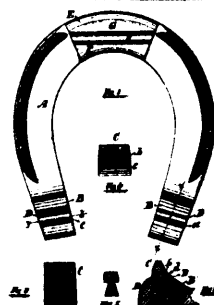
8511 L. Day's Improvements in Horse Shoes.
