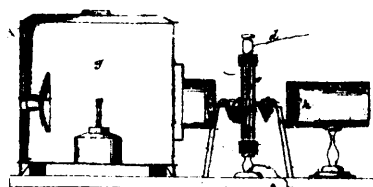
2177 Highton's Improvements on Electric Telegraphs.
