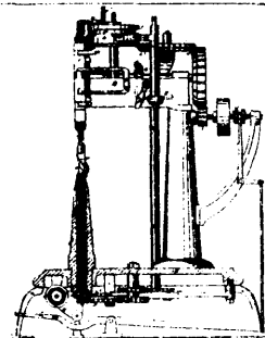
2183 Sheffield &amp; Mellor's Machine for Sewing Leather.
