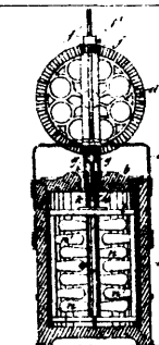
2180 Wattles &amp; Cable's Clarn.
