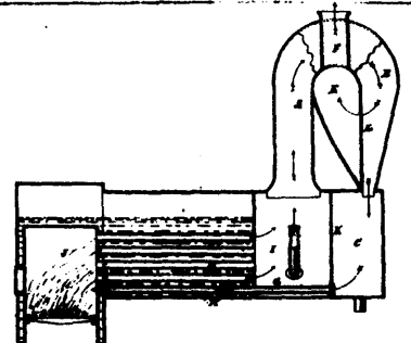
3810 Ferrard's Spark Arrester.
