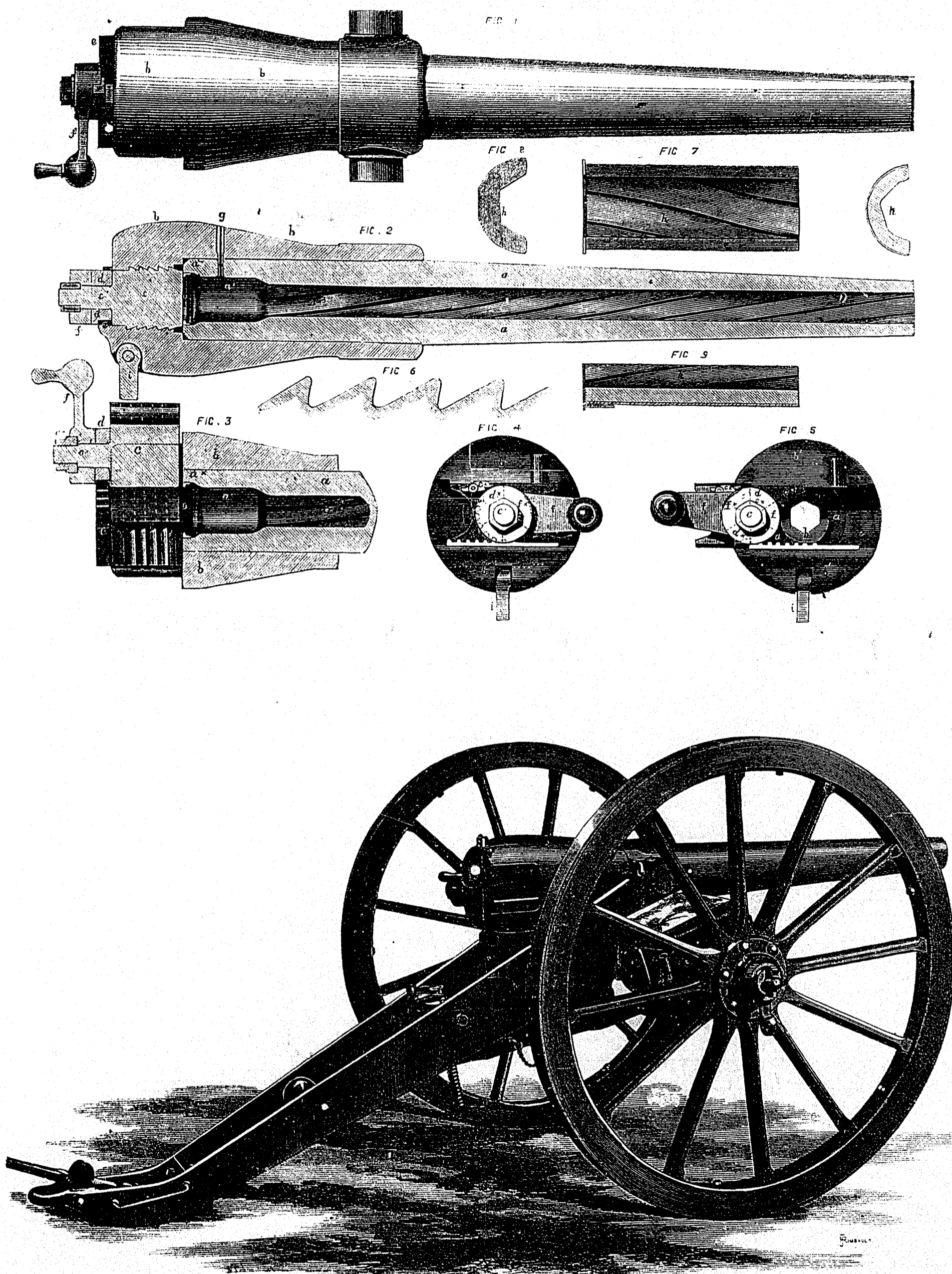
THE WHITWORTH 9-POUNDER BREECH-LOADING RIFLED FIELD GUN.
