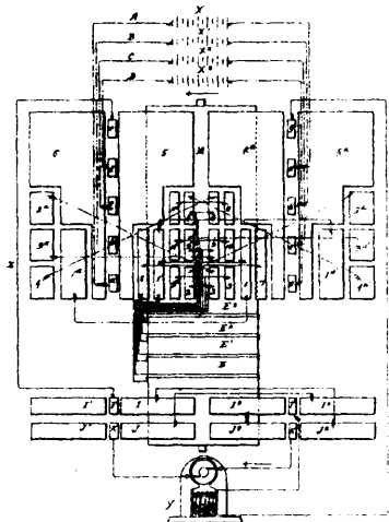
Rae's Controlling Switch for Electric Railways.
