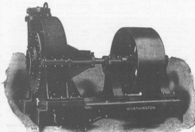
TEN INCH TURBINE DREDGING PUMP.
