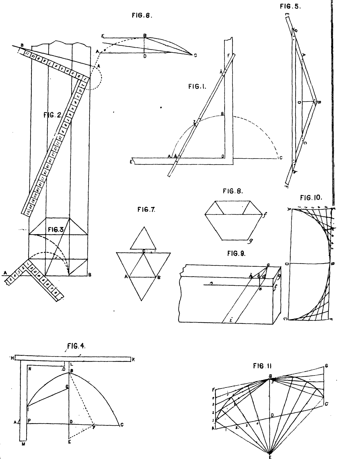
EXAMPLES OF THE PRACTICAL USE OF THE STEEL SQUARE. BY F. T. HODGSON, ACHT., ED. "AMERICAN BUILDER," (LATE OF COLLINGWOOD, ONT.)
