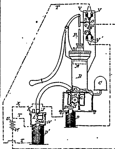
24312 Worth's Electric Air pump
