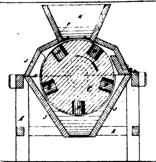
12299 Wilson's Improvements on Grain Trollers.
