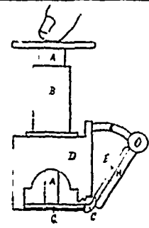
6104 Hawthorn's Improvements on Hand Stamps.
