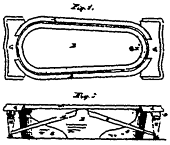
6121 Johnston & Taylor's Improvements on Portable Baths.
