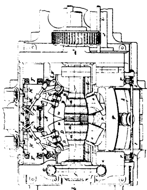
39566 Barraclough's Machinery for Shaping, Finishing and Flanging Metal Bodies for Barrels, etc.
