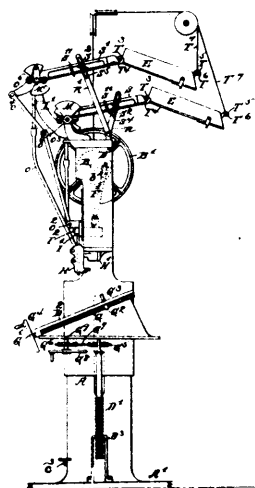
39568 Doig's Box-nailing Machine.
