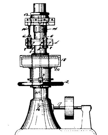
39562 Doig's Nailing Machine.
