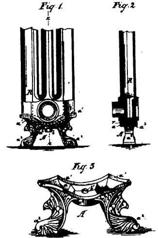
34175 Tomkins & Williams' Radiator.
