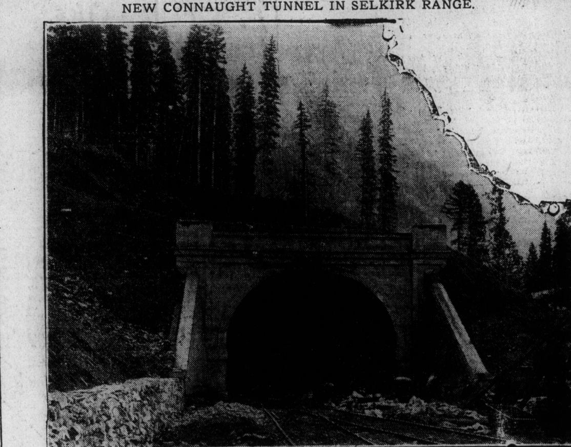
The new Connaught tunnel which pierces Mt. Macdonald in the Selkirk Range is a marvellous engineering feat. The tunnel was cut through five miles of solid rock and saves miles of snowsheds and curves. Photo shows the entrance to the tunnel with the mountain in the background.
