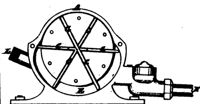
3559 Barnes' Rotary Pump.
