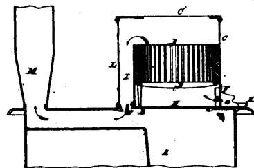
3564 Chamberlain's Portable Furnace.
