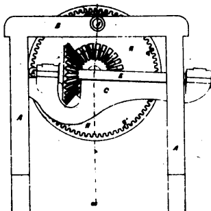
3566 Clokey's Threshing Machine Safety Gear.
