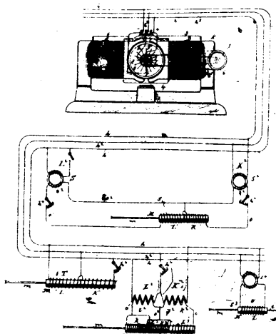
35455 Van Depoele's Pulsating Current System.
