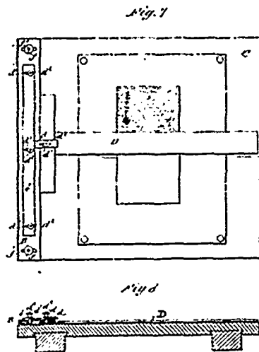
25380 Podgorski's Scale Divider.
