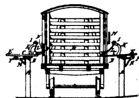
14267 Tingley's Improvements in Devices for Feeding and Watering Stock in Cars.
