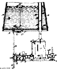
14266 Beach's Improvements on Systems of Water Works.
