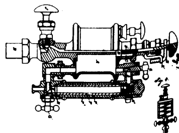
14270 McCoy's Improvements on Lubricators.
