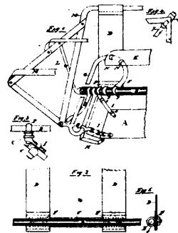
14261 McCrea's Improvements in Carriages.
