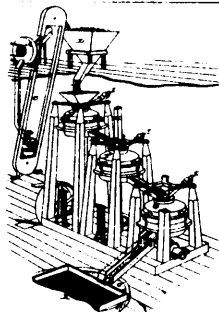
14265 Eichelberger's Improvements on Process and Mode of Manufacturing Pulp.
