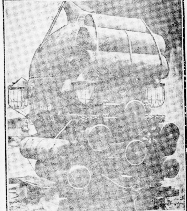
Just as useful as it is queer looking is this modern diving bell undergoing repairs in a shipyard at New York. Divers work from the big chamber which is attached to a sunken craft while salvage operations were in progress
