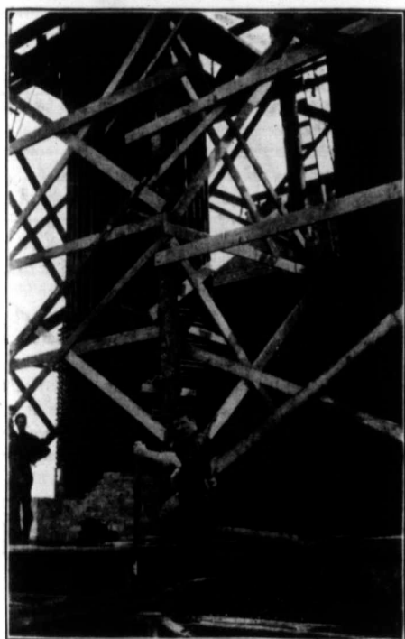
Bettington Boilers of Waterford Lake power-house, in course of construction.
