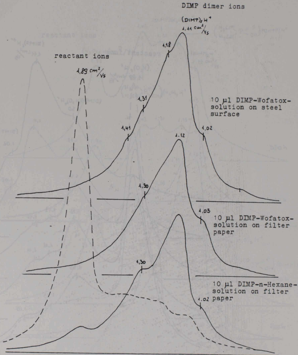
Fig. 7: Simulation of wipe-tests on a steel surface contaminated with Wofatox-DIMP-solution of a concentration of 0,1 µg DIMP / ml solution, the DIMP content was about 1 µg in all tests
