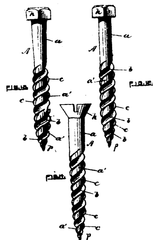
32653 Rogers' Wood Screw, etc.
