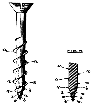
32651 Rogers' Wood Screw.
