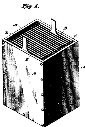
32655 Dey's Storage Battery.
