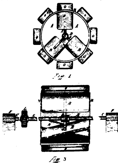
33877 Mutter's Water Motor.
