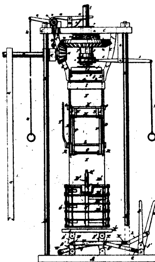
19661 Battson's Press for Sacking Bran, &amp;c.
