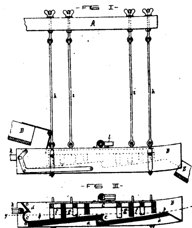
19656 Moon's Ore Amalgamator.
