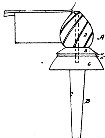
16849 Bourgeois's Improvements on Heel Burnishing Tools
