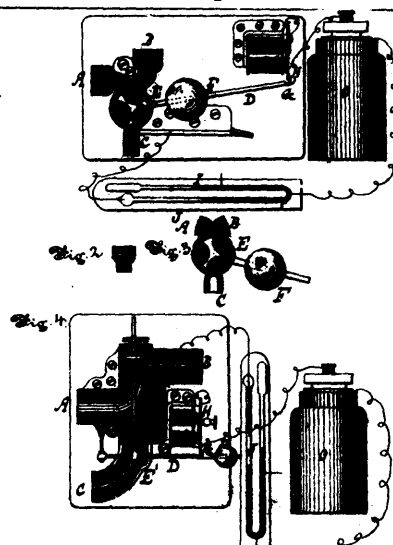
16857 Buxton and Ross's Means for Regulating the Supply of Water to House Service Pipes and Cisterns.
