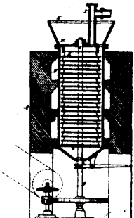
14435 Stormer's Apparatus for Drying and Distilling Spent Dye Wood and Saw Dust, &amp;c.
